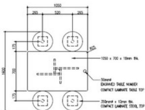
PLAN OF TABLE & STOOLS - SEATING ARRANGEMENT TYPE 2
