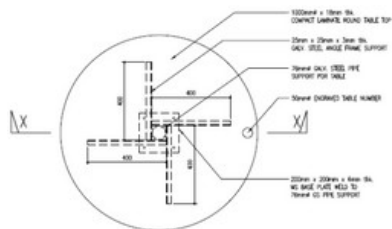
PLAN DETAIL OF BRACKET FOR FIXING OF ANGLE FRAME TO TABLE TOP
